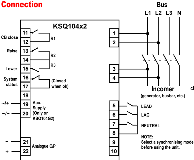
System "P" "Spot-on" synchronising LEAD direction
