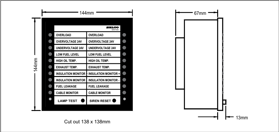
Fig. 6. Dimensions.
